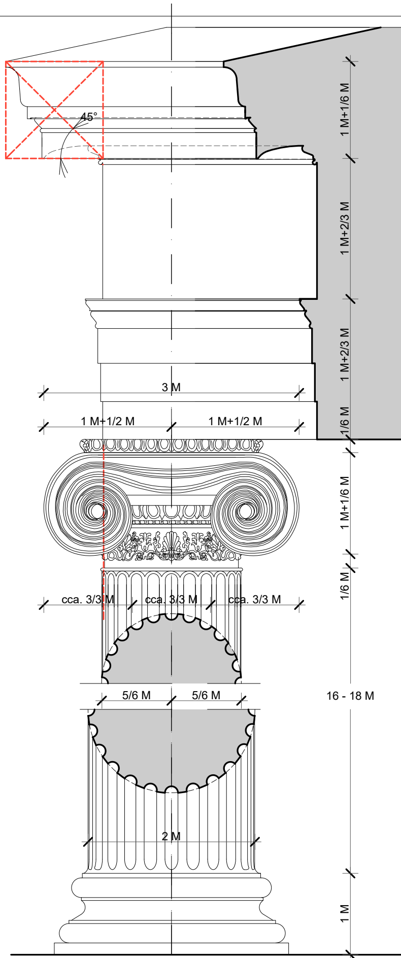
ATTIC IONIC ORDER
